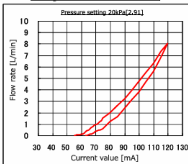
Voltage-current characteristics
